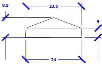
PC24-5 1 mold compatible with S7-2
