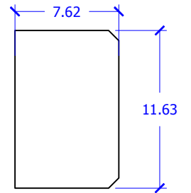
L12-4 2 at 96 chamfer ends
